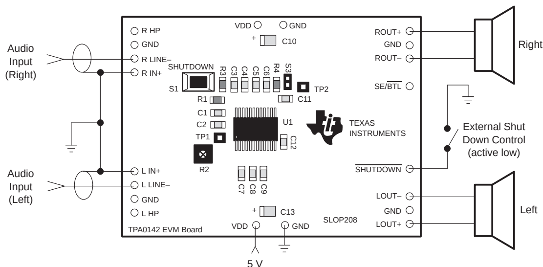
Figure 3–9. TPA0142 EVM Connected for Stereo BTL Output
