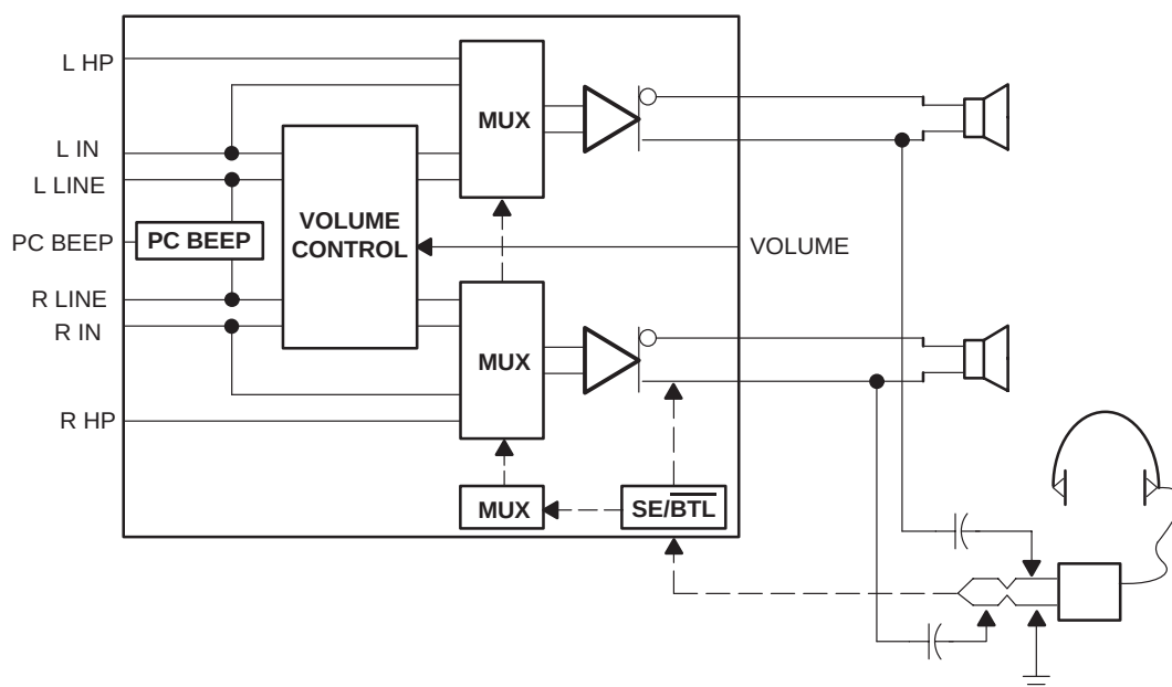
Figure 3–4. TPA0142 Amplifier IC
